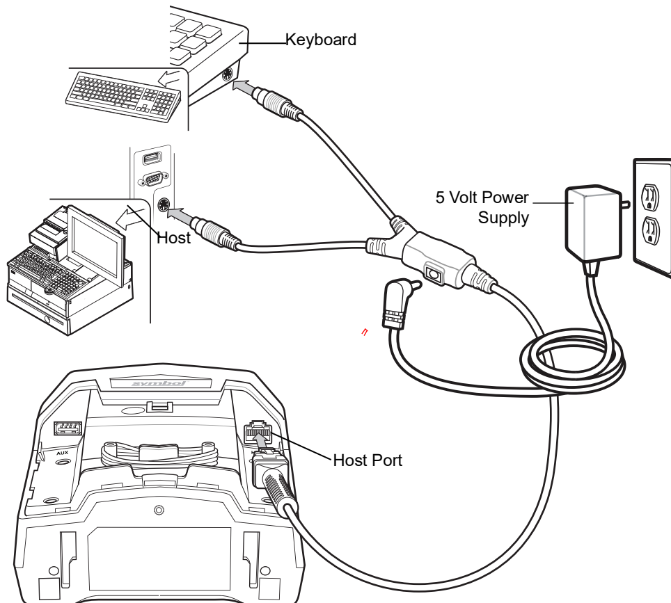
Figure 10-1 Keyboard Wedge Connection - 5 Volt Power Supplied Externally
