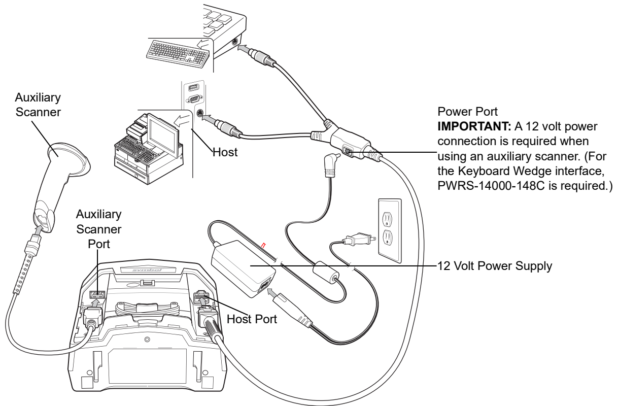
Figure 10-2 Keyboard Wedge Connection - With Auxiliary Scanner/Power Supplied Externally
