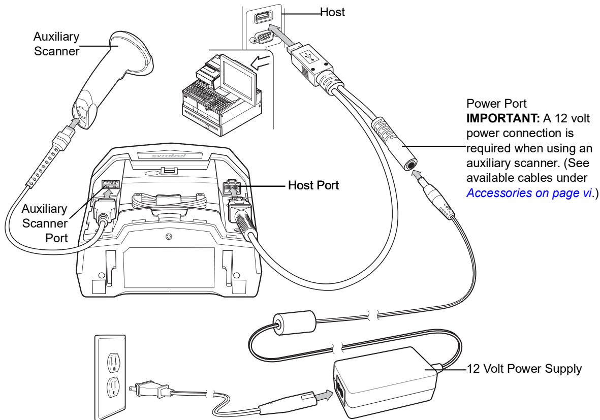
Figure 7-2 USB Connection With Optional Auxiliary Scanner - 12 Volt Power Supplied Externally
