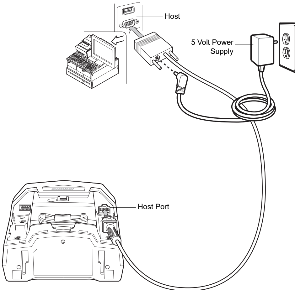
Figure 8-1 RS-232 Connection - 5 Volt Power Supplied Externally
