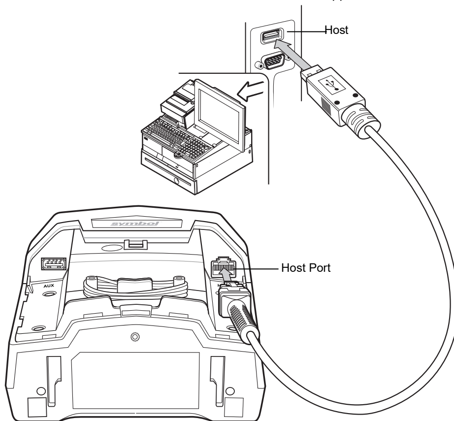
Figure 7-1 USB Connection - Host Supplies Power
