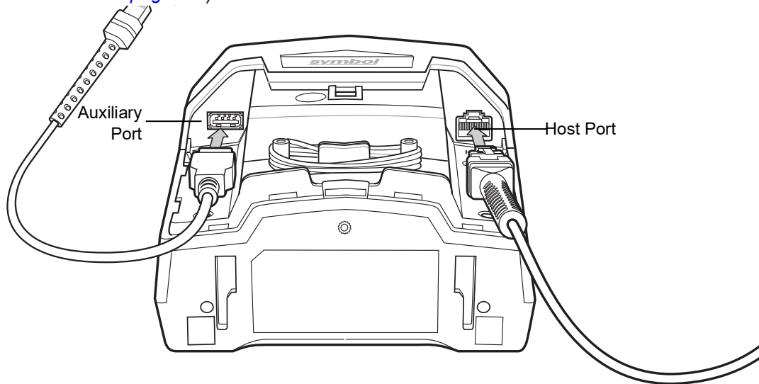
Figure 1-6 Installing Cables
