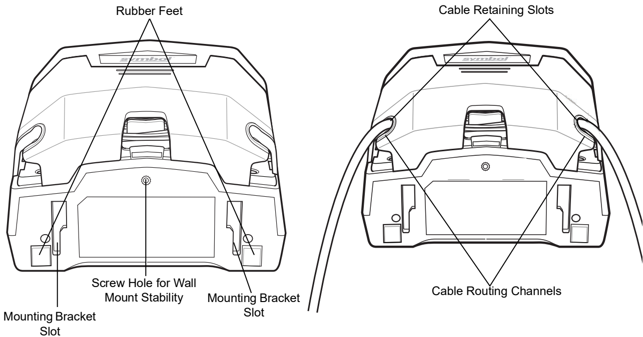
Figure 1-3 DS7708 Views - Bottom and With and Without Cables
