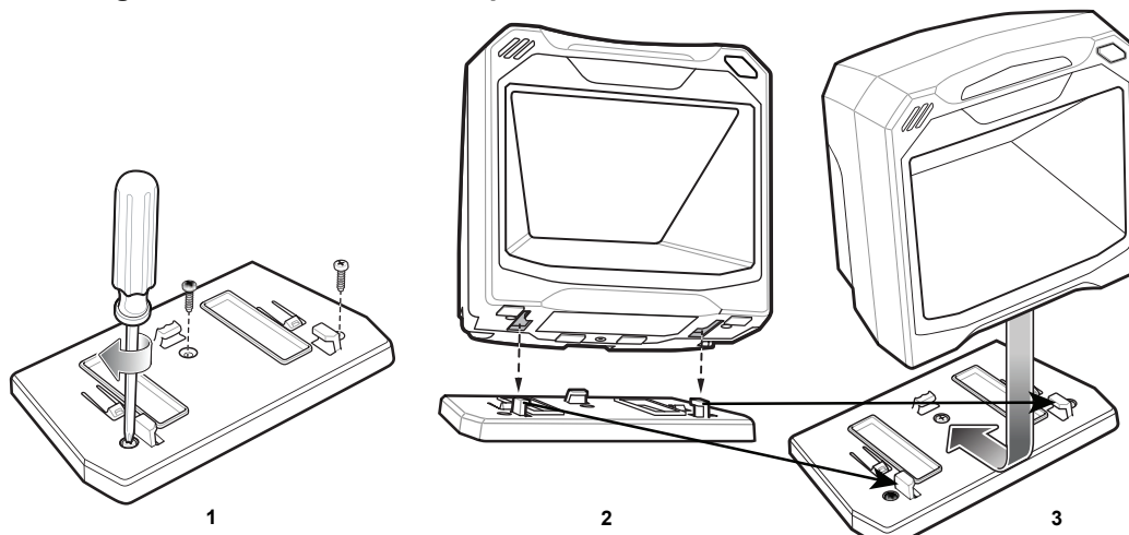
Figure 1-10 Table Top Mounting Diagram
