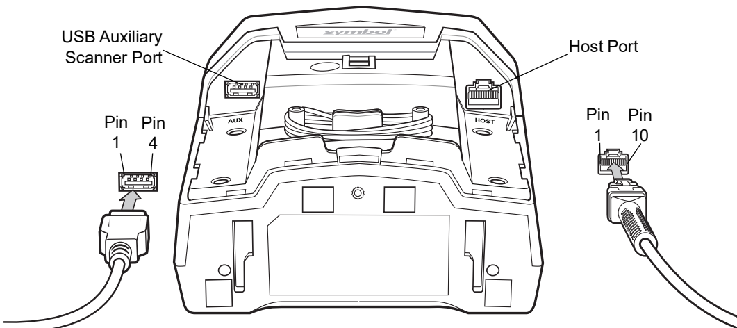
Figure 4-1 Cable Pinouts
