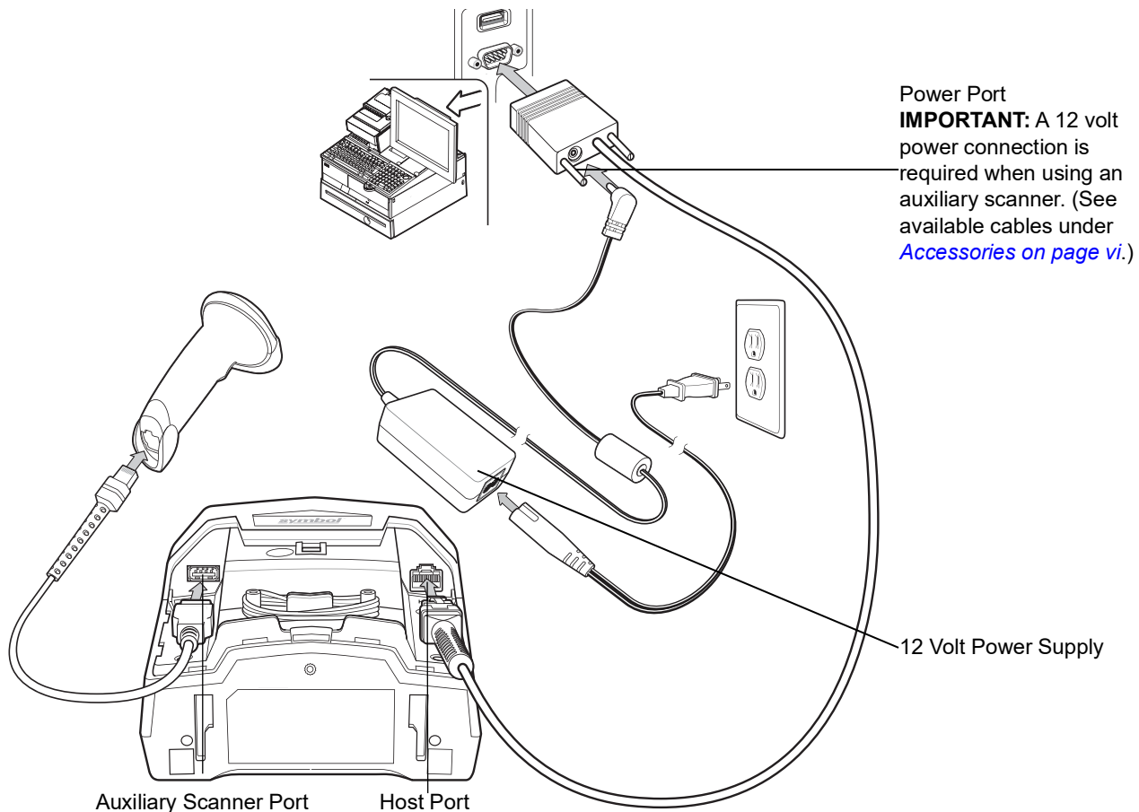
Figure 8-2 RS-232 Connection with Auxiliary Scanner - 12 Volt Power Supplied Externally
